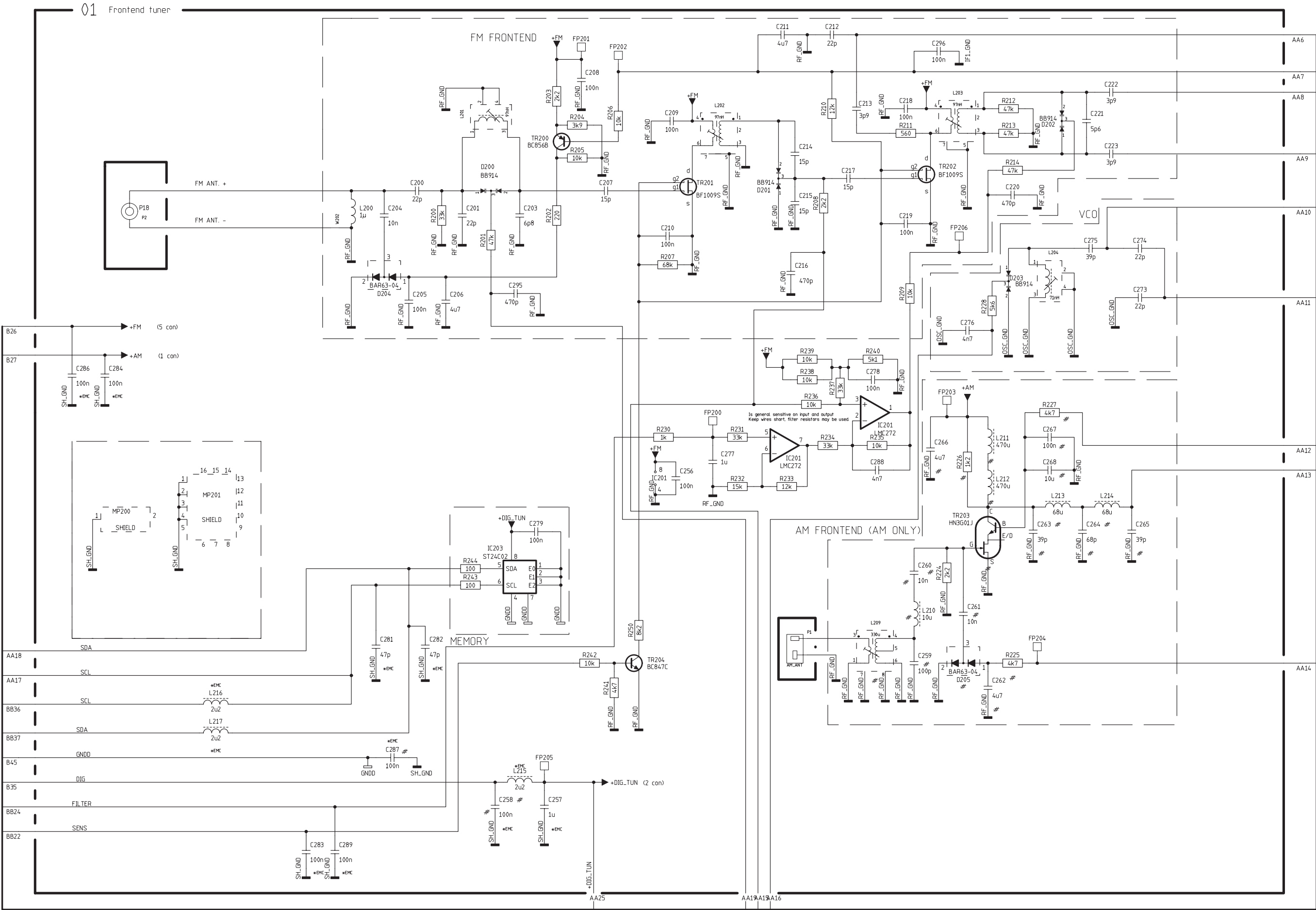
DIAGRAM A – Frontend tuner PCB drawing for PCB1 see page 2.15
