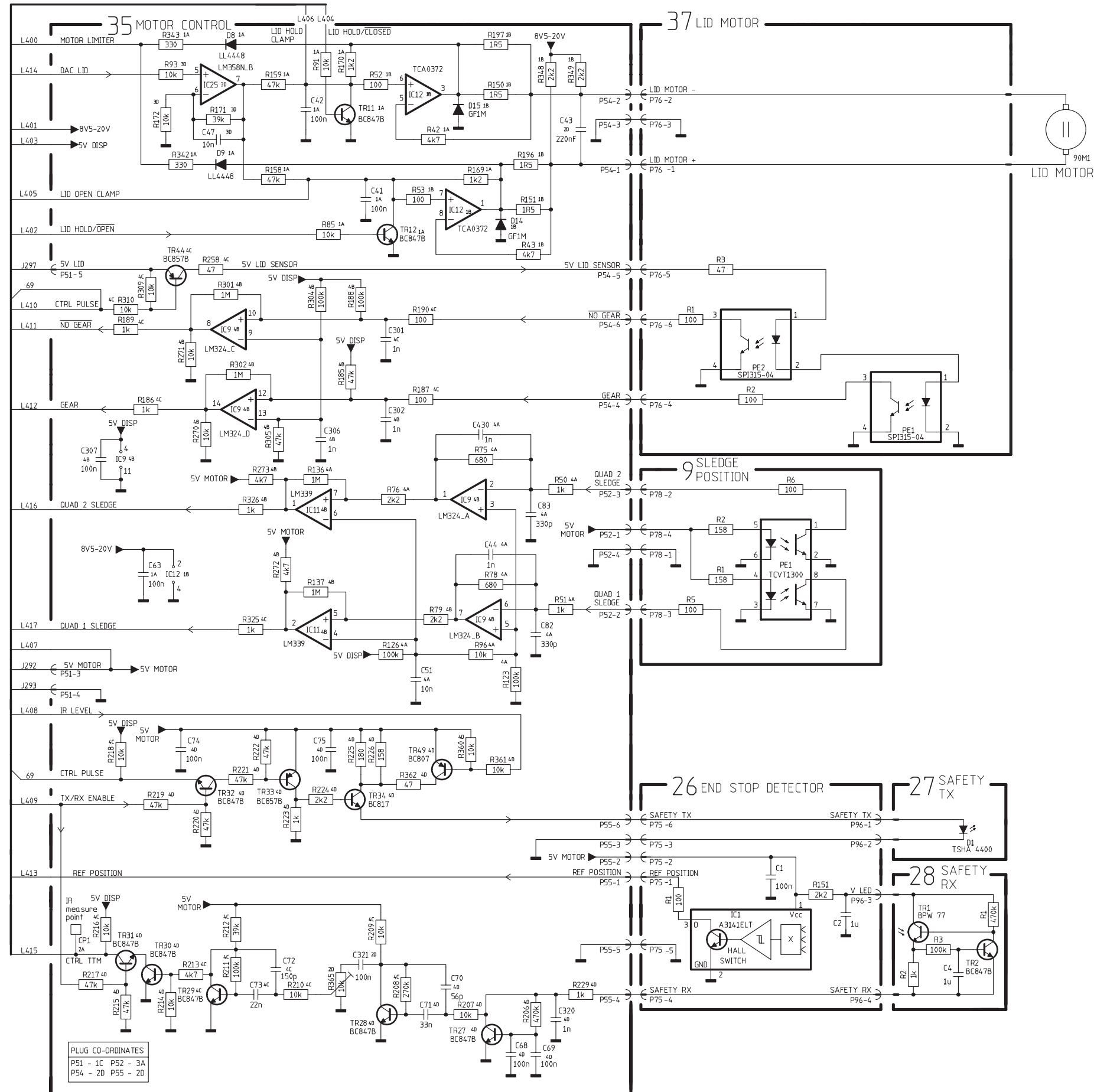
PCB drawing for PCB35 see page 2.27
