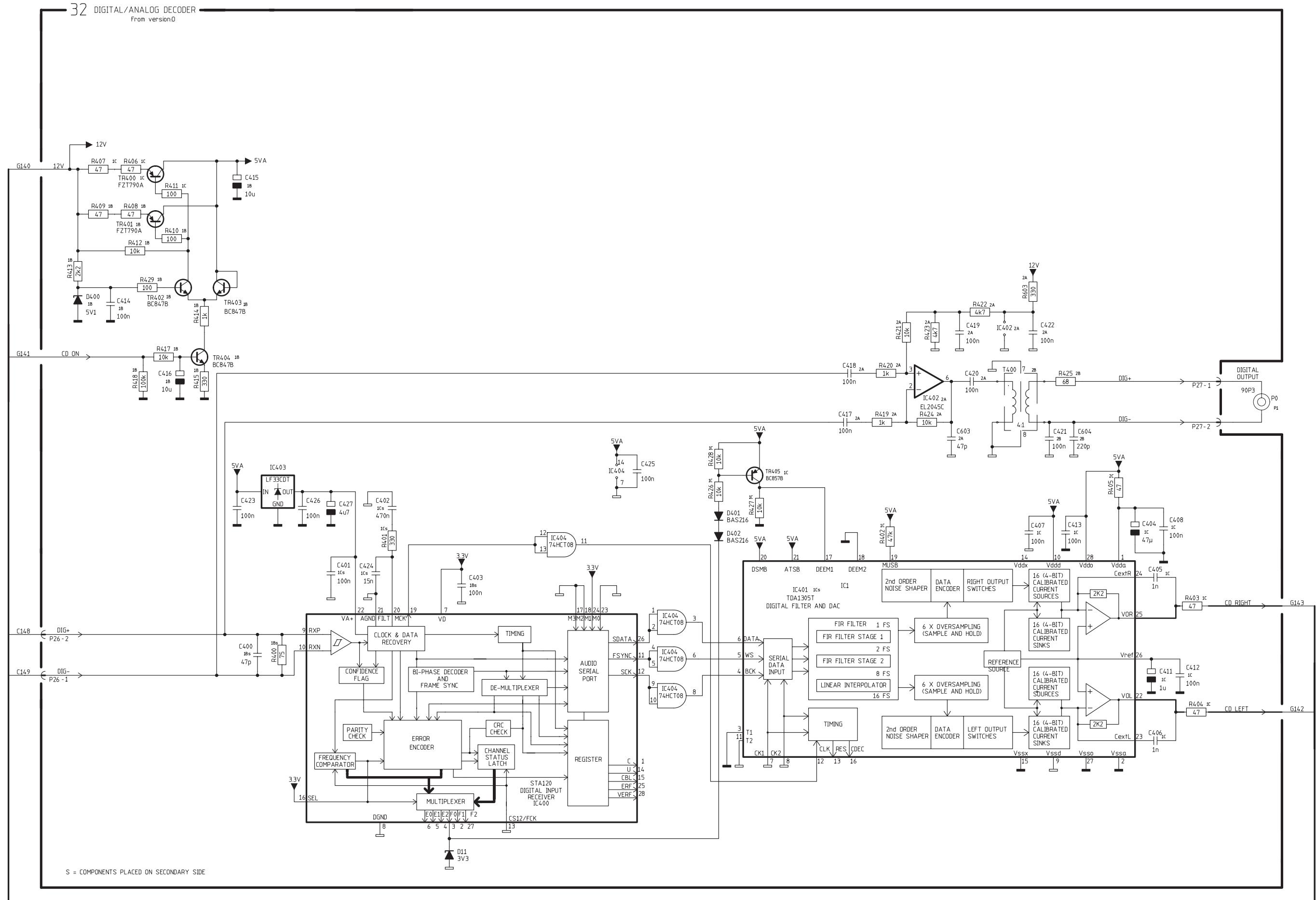
PCB drawing for PCB32 see page 2.21
