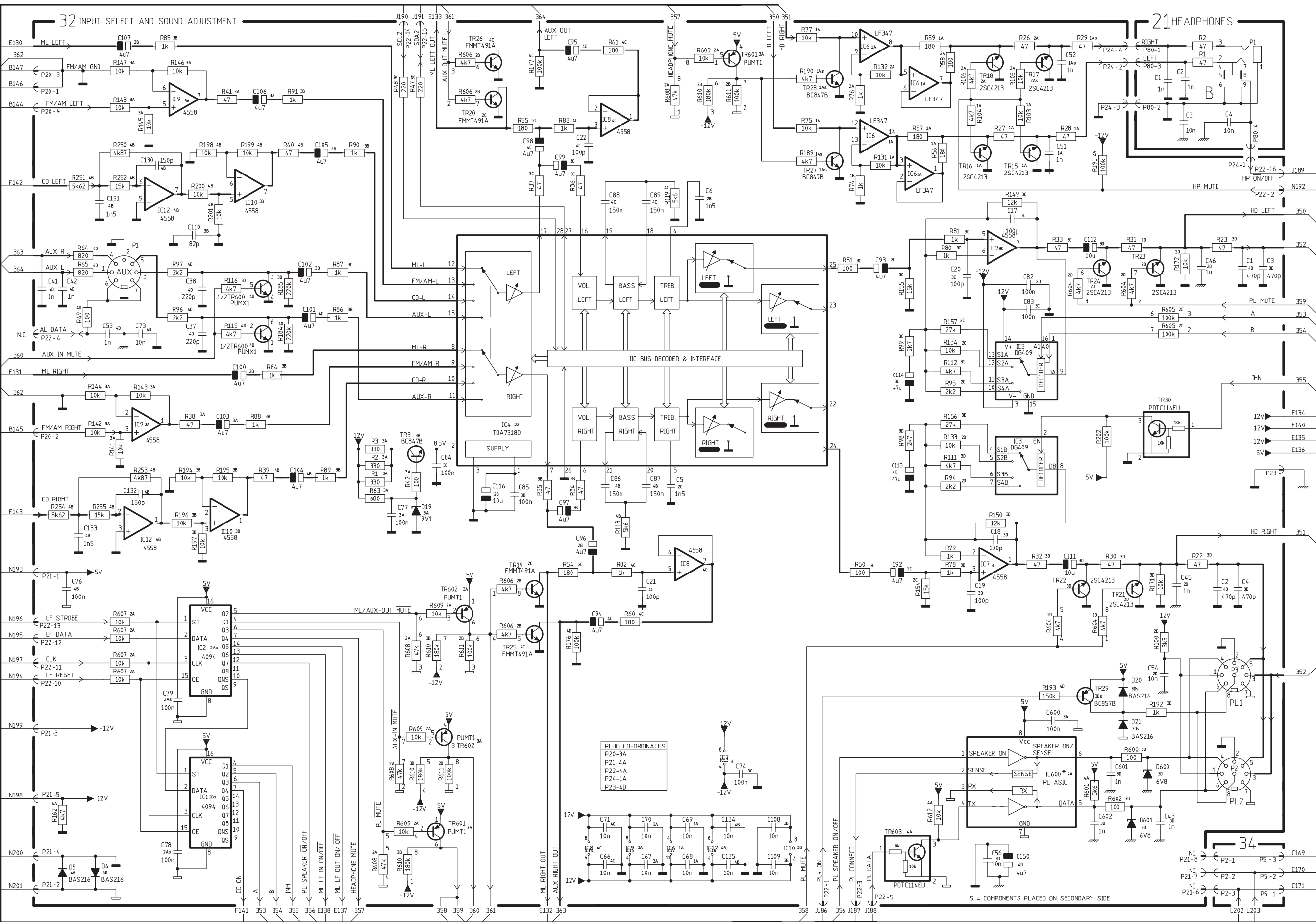
DIAGRAM G – Input select and Sound adjustment PCB drawing for PCB21 and PCB32 see page 2.21
