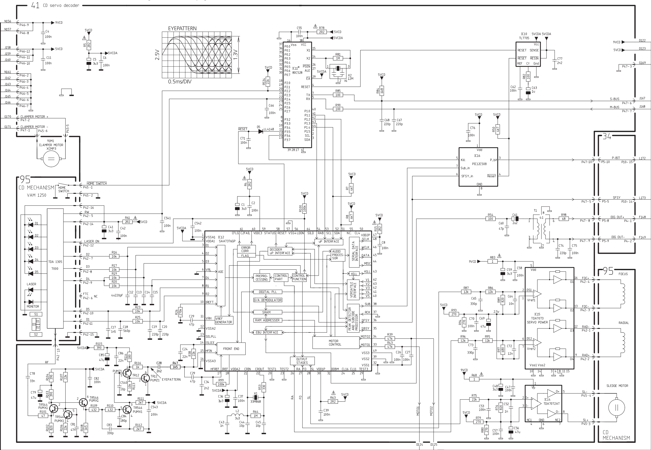
DIAGRAM C – CD servo decoder PCB drawing for PCB41 see page 2.17
