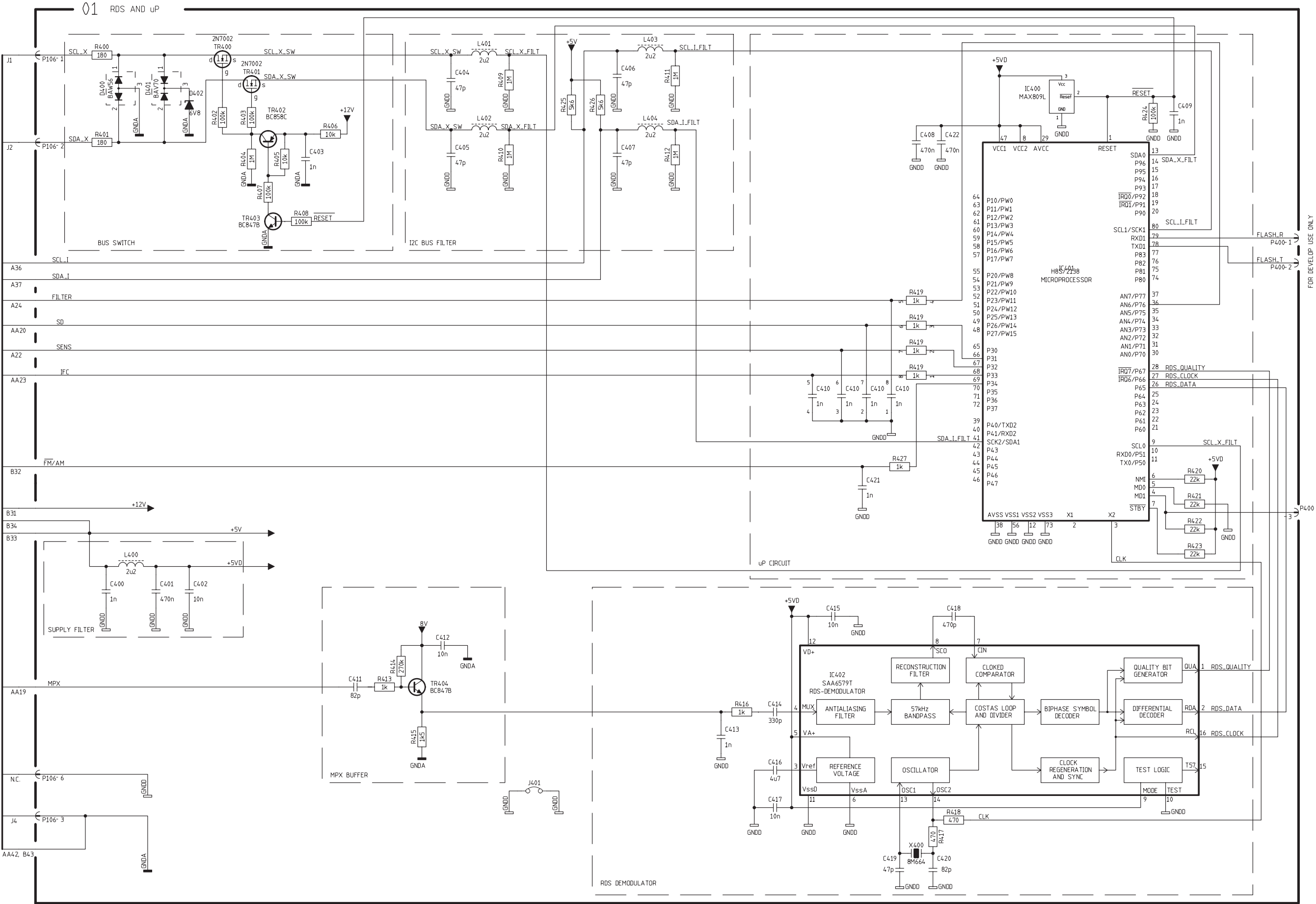
DIAGRAM BB – RDS and \mu P PCB drawing for PCB1 see page 2.15
