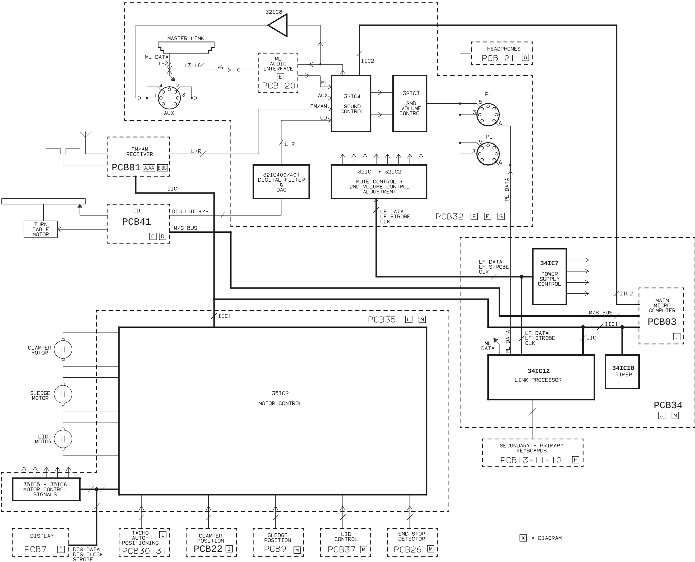
Overall block diagram
