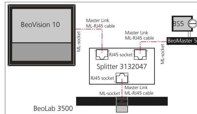
Master Link
